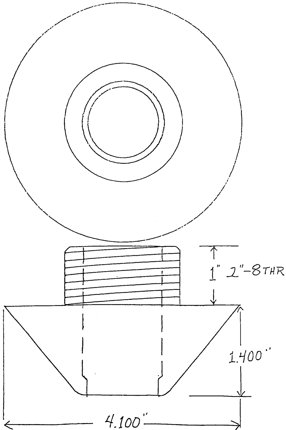
STANDARD SHALLOW BASIN (SPRUE DIA.: 1 1/4" DIA.) (PART NO. 31055P)
