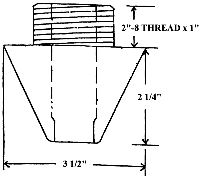
ROUND DEEP POURING BASIN (SPRUE DIA.: 5/8"; 3/4"; 7/8"; and 1") (PART NO. 32043P; 32035P; 32045P; and 32055P respectively)
