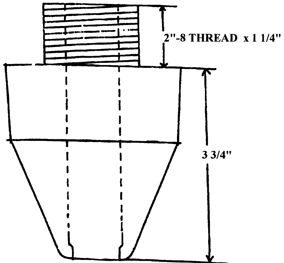
ROUND DEE POURING BASIN (SPRUE DIA.: \frac{5}{8}" ; 1" & 1 \frac{1}{2}" ) (PART NO.: 90420-099 & 9420-133 respectively) (OPTIONS: \frac{7}{8}" SPRUE DIA.)
