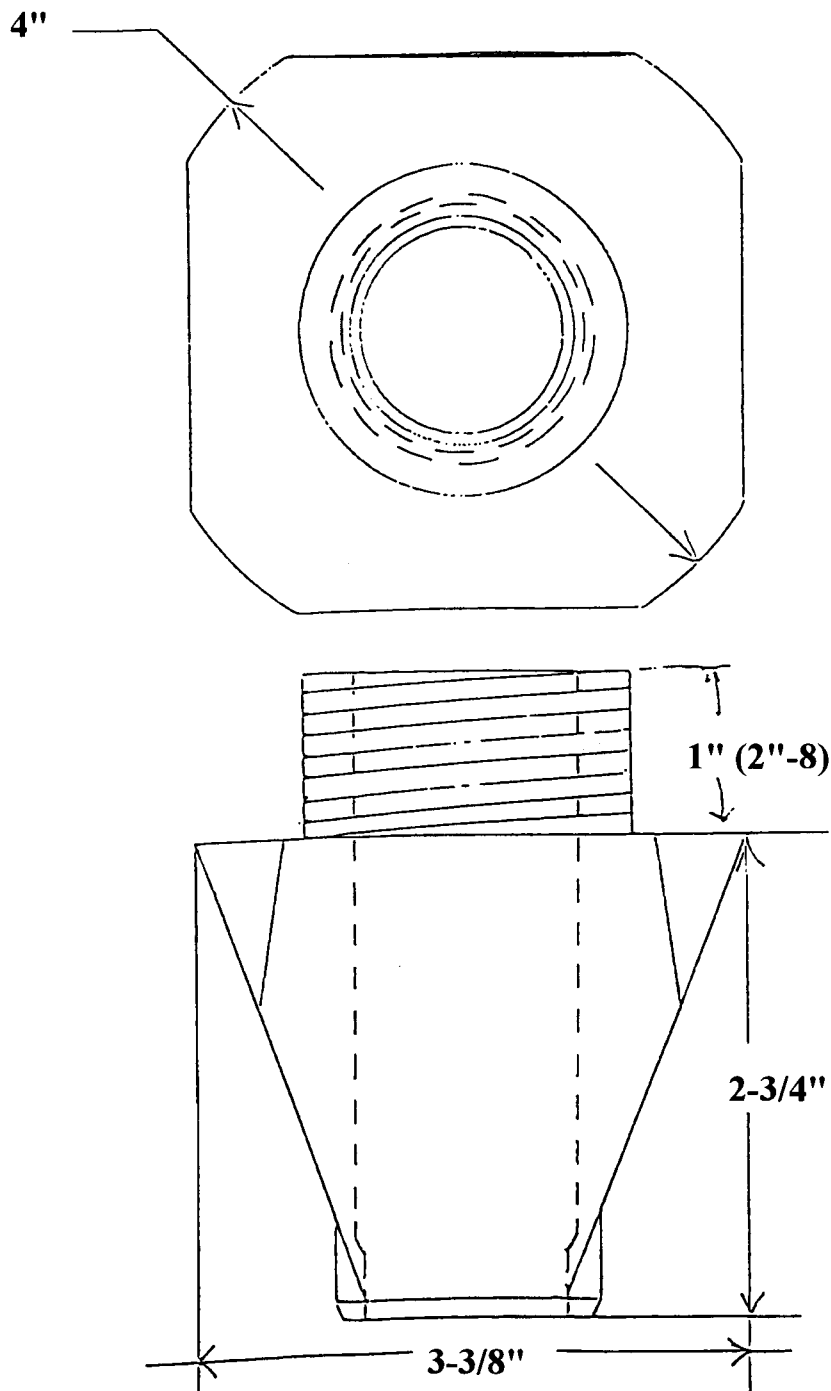
3-3/8" DEEP PYRAMID BASIN WITH REINFORCED NOSE (SPRUE DIA. 1 1/4") (PART NO. 210315P)
