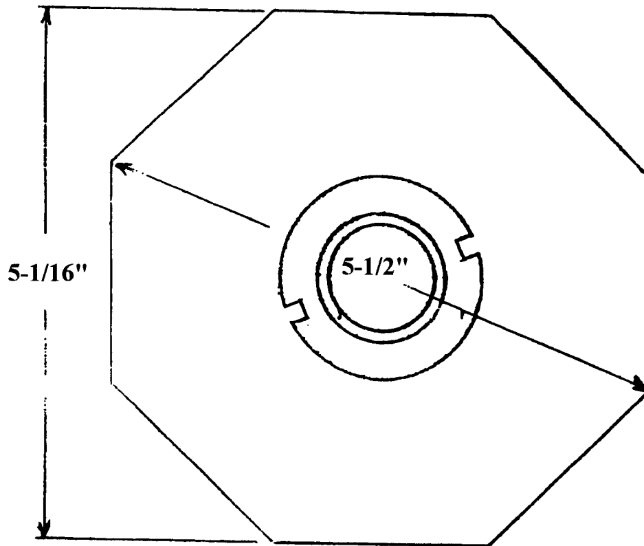
25 mm. - 8 SIDED POURING CUP 5-1/2" BASE WITH M-48 THREAD PART NO.: 210330P
