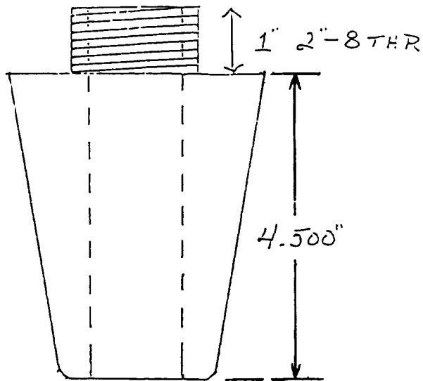
ROUND FOUR LOOP BASIN (SPRUE DIA. 1 1/2") (PART NO. 32090P) (OPTIONS: SPRUE DIA.: 1" 1 1/4")
