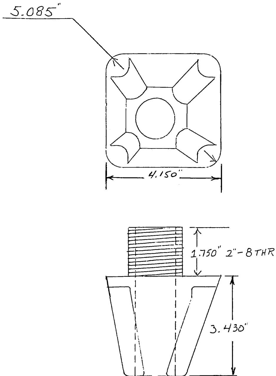
SQUARE FOUR LOOP BASIN (SPRUE DIA. 1"; 1 1/4"; and 1 1/2") (PART NO.: 32102P; 32101P; and 32100P respectively)
