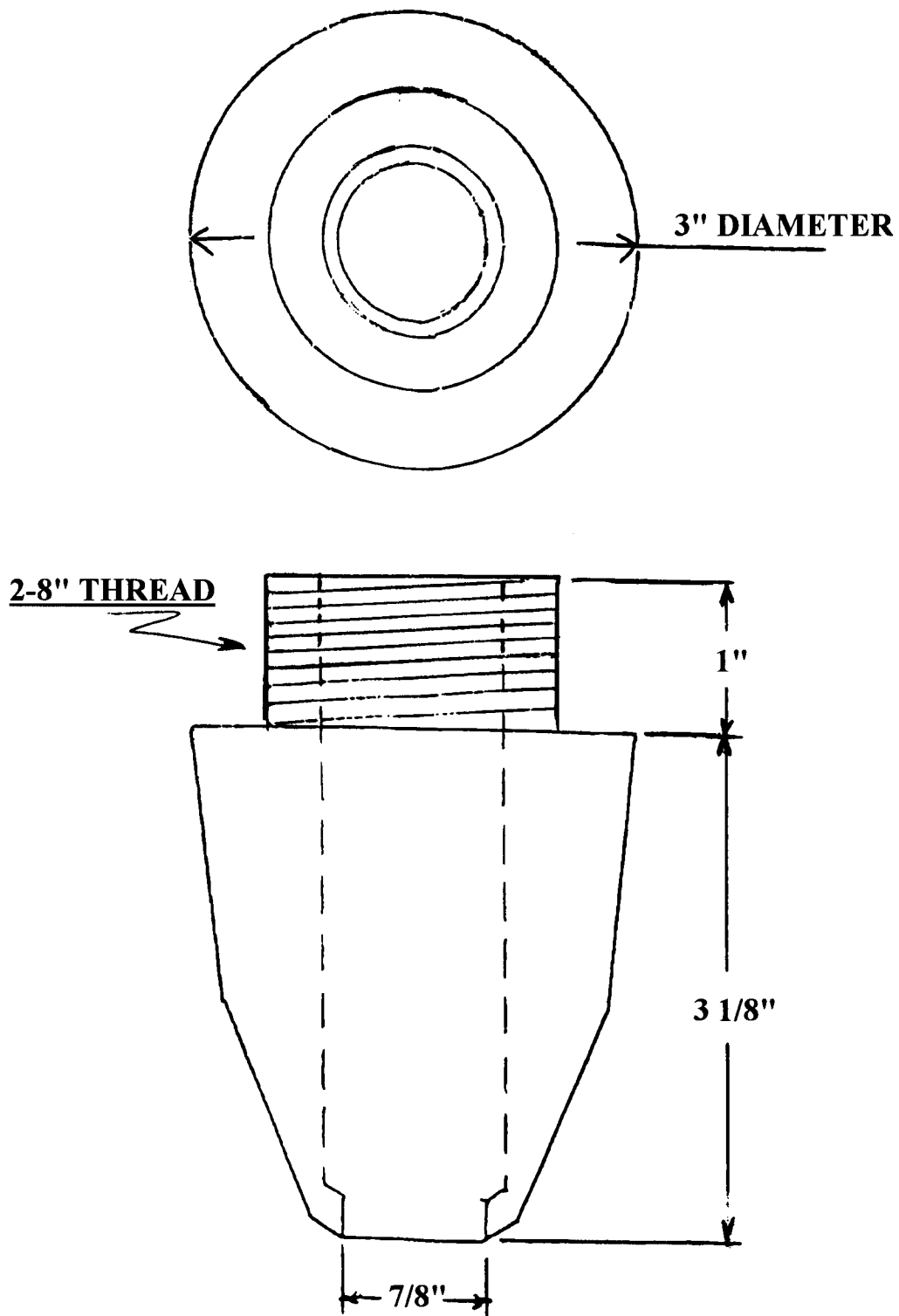
LARGE ROUND STRAINER CORE BASIN [SPRUE DIA. 7/8"; (PART NO. 210300P)] (OPTIONS: 1" SPRUE DIA. & M-48 THREAD) (ALSO 1" & 1-1/4" SPRUE DIA. & 2"-8 THREAD)
