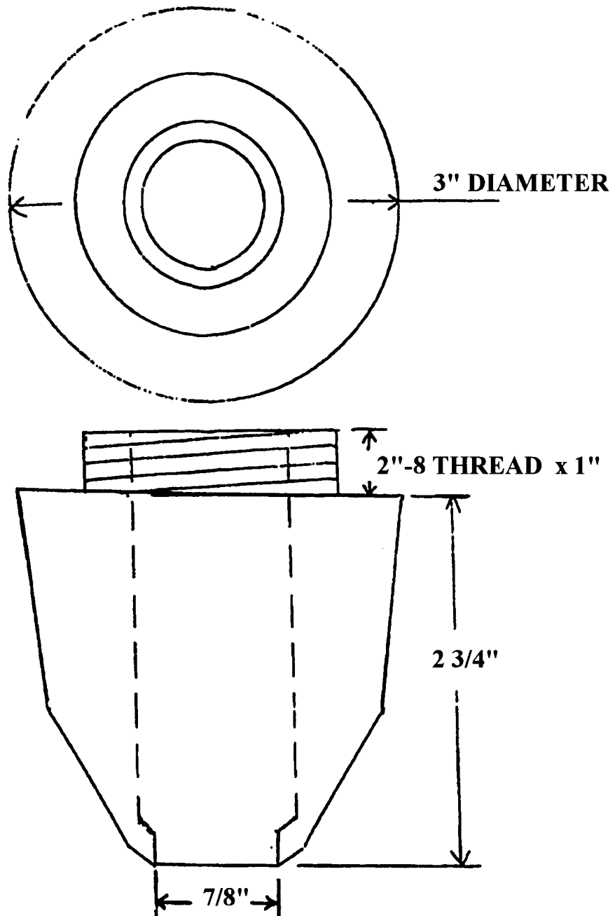
SMALL ROUND STRAINER CORE BASIN [SPRUE DIA. 7/8"; (PART NO. 210302P)] (OPTIONS: 1" SPRUE DIA. & M-48 THREAD) (ALSO 1" & 1-1/4" SPRUE DIA. & 2"-8 THREAD)
