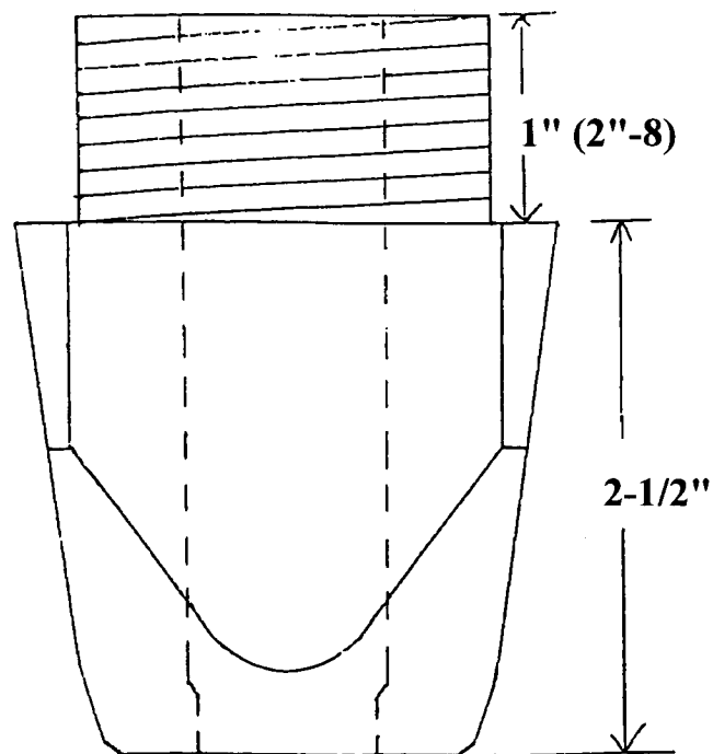
SMALL SQUARE STRAINER CORE BASIN (PART NO. 210316P: 1-1/4" SPRUE DIA.; PART NO. 210318P: 1" SPRUE DIA. ) (PART NO. 210326P: 1-1/2" SPRUE DIA.) (OPTIONS: 5/8" & 7/8" SPRUE DIAMETER)
