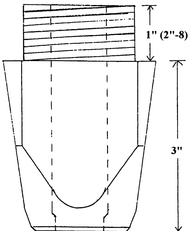
LARGE SQUARE STRAINER CORE BASIN (PART NO. 210317P: 1-1/4" SPRUE DIA.; PART NO. 210319P: 1" SPRUE DIA.) (PART NO. 210327P: 1-1/2" SPRUE DIA.) (OPTIONS: 5/8" & 7/8" SPRUE DIAMETER)
