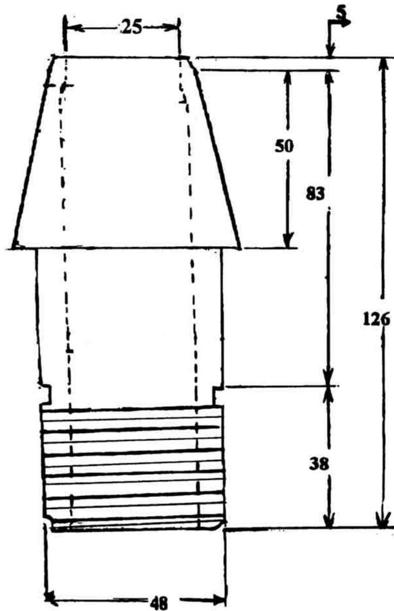
25MM BASIN FOR LONG WELL - PART NO. 501029
