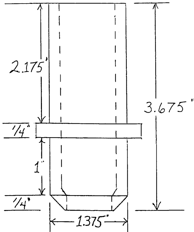
BASIN LINER (SPRUE DIA. 7/8") (PART NO.: 33020P)
