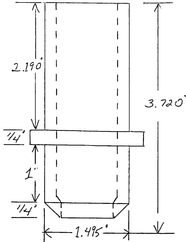
BASIN LINER (SPRUE DIA. 1") (PART NO.: 33030P)
