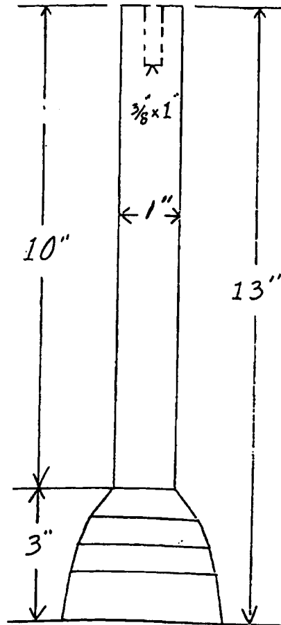
1" POP UP DOWN SPRUE (PART NO. 210235P) (OPTIONS: 3/4" & 7/8" DIAMETER)
