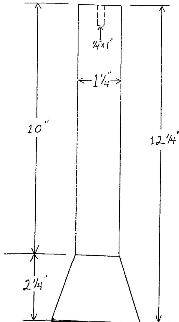
1 1/4" POP UP DOWN SPRUE (PART NO. 210230P)
