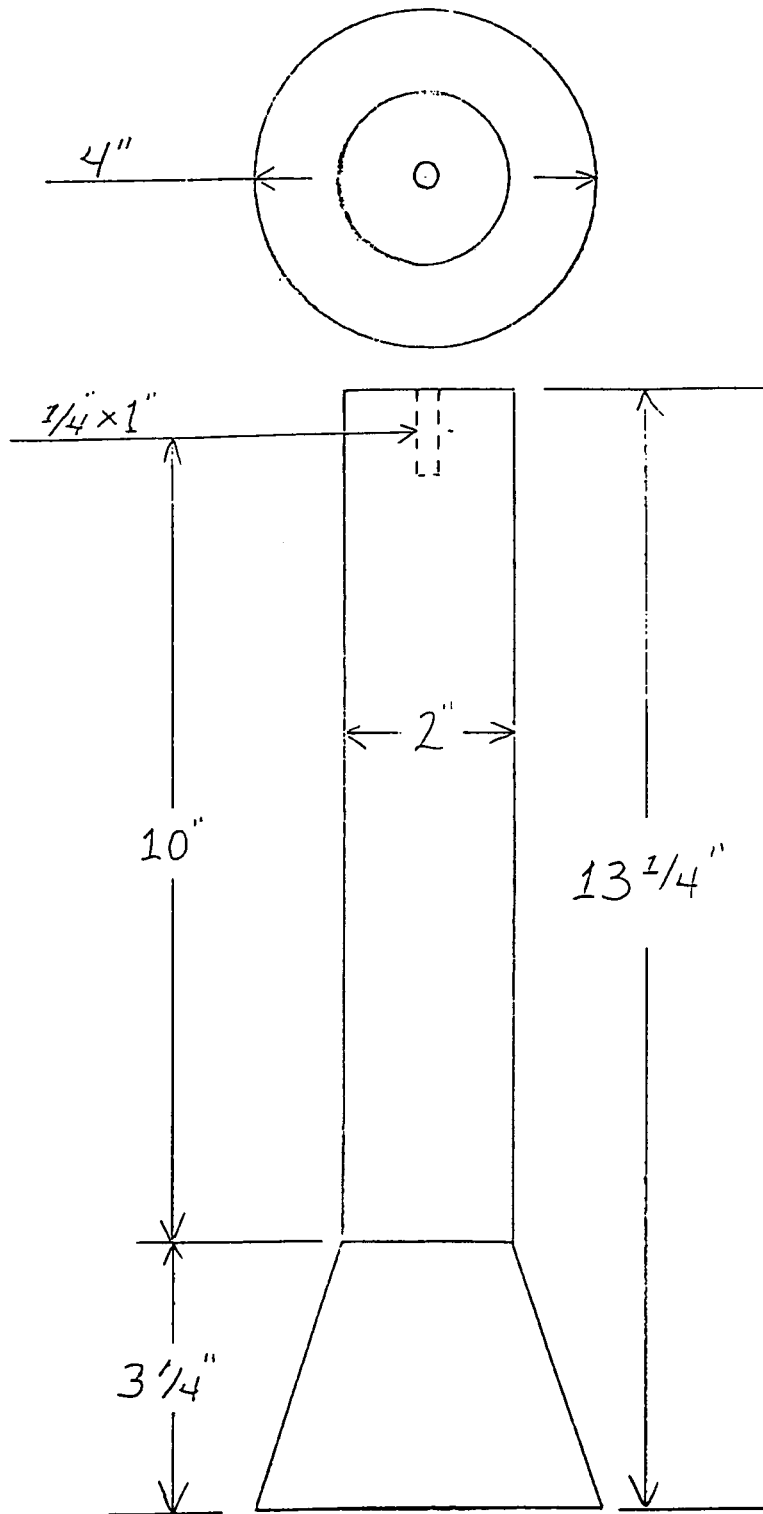
2" POP UP DOWN SPRUE (PART NO. 210242P)
