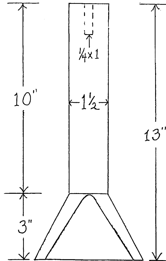
1 1/2" POP UP DOWN SPRUE W/ 1 FLAT SIDE (PART NO. 210243P)
