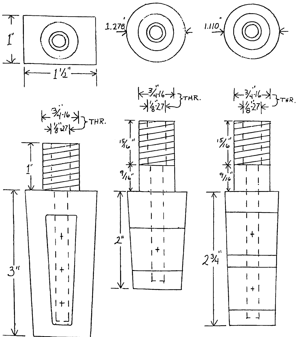
(1) RECTANGULAR TRIPLE BLADDER (2) ROUND SINGLE BLADDER (3) ROUND DOUBLE BLADDER PNEUMATIC STEEL CORE LIFTERS WITH RUBBER BLADDERS
