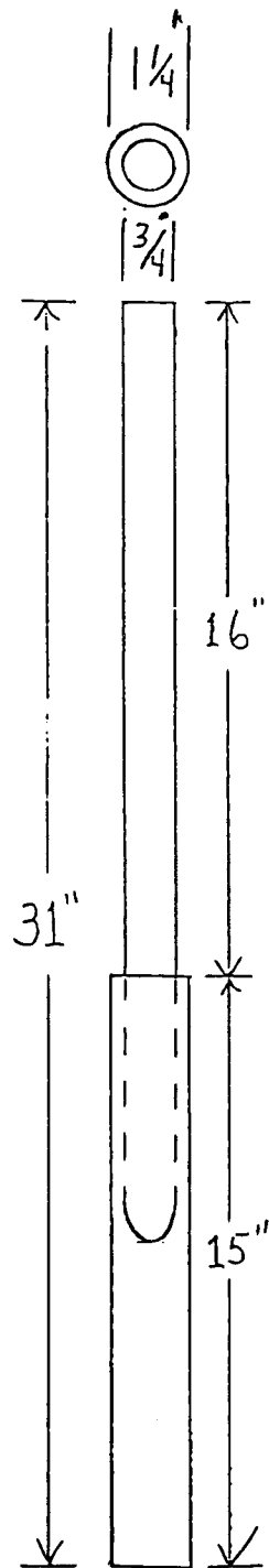
DUMMY DIGGER SPECIAL STEEL ROD WITH ONE END CAST URETHANE (PART NO. 90800-140)
