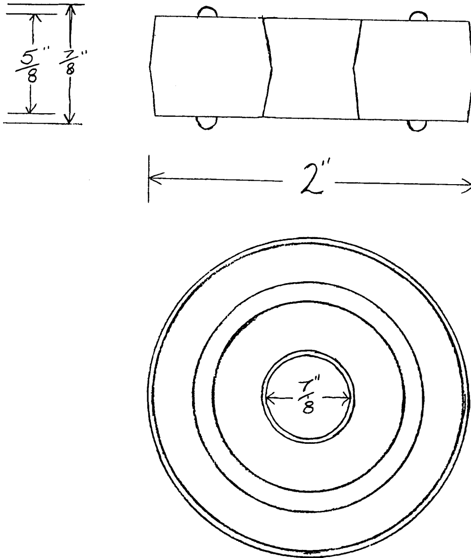
RUBBER SEALING RING PART NO. 15020S U-180 2"OD. X \frac{7}{8}" ID. 50-60 DURO-RUBBER
